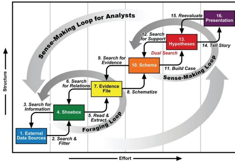
Fig. 2. Adapted from sensemaking loop, Pirolli and Card [21]
